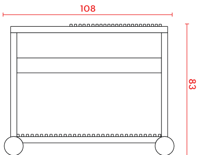
VISTA FRONTAL
