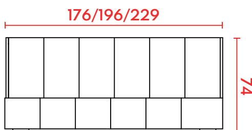
VISTA FRONTAL
