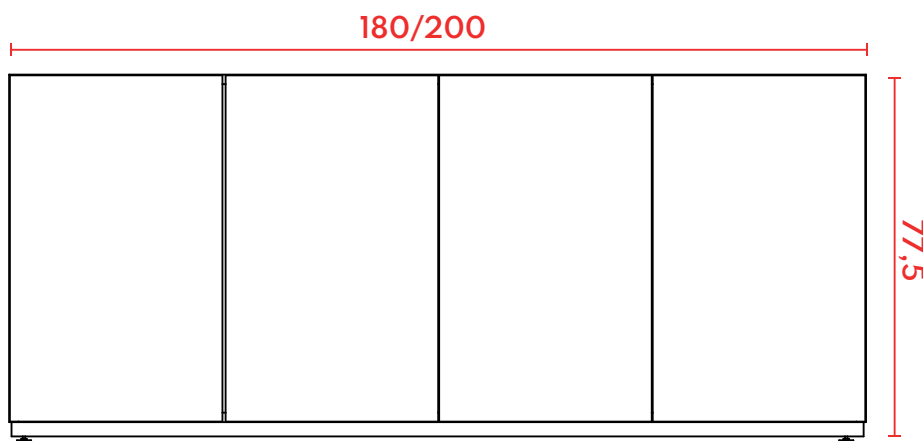
VISTA FRONTAL
