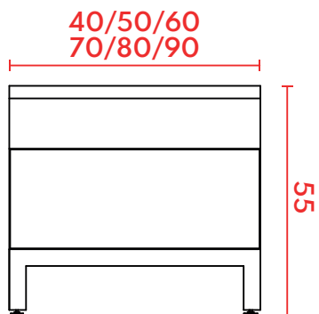
VISTA FRONTAL
