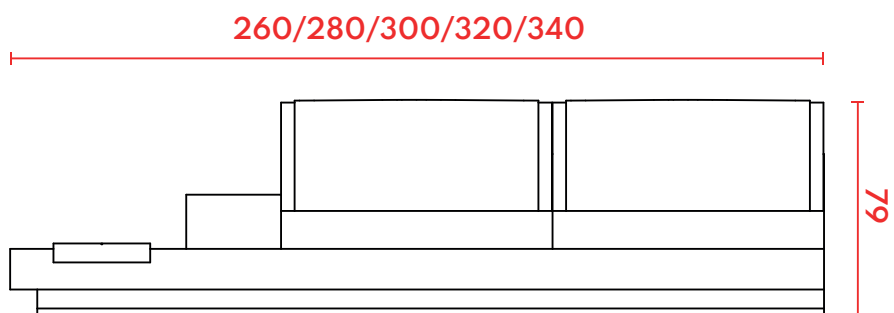
VISTA FRONTAL
