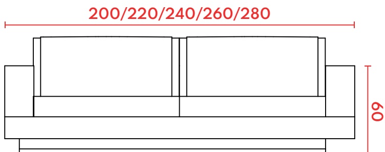
VISTA FRONTAL
