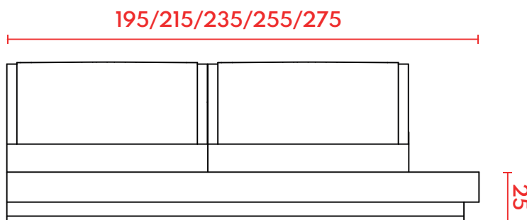
VISTA FRONTAL
