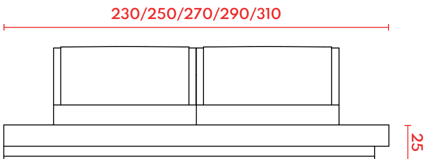
VISTA FRONTAL
