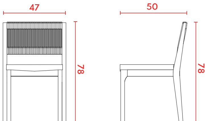
VISTA FRONTAL
