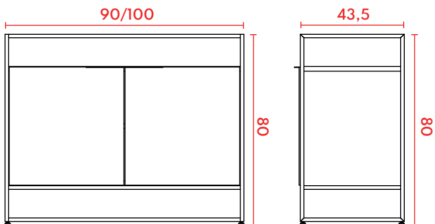
VISTA FRONTAL
