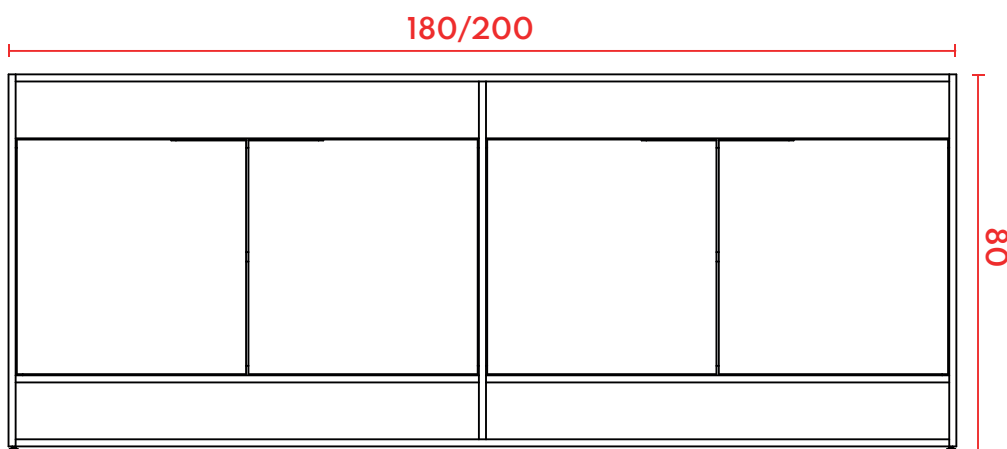
VISTA FRONTAL
