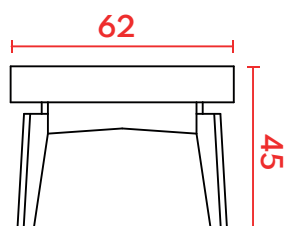
VISTA FRONTAL
