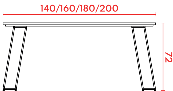
VISTA FRONTAL
