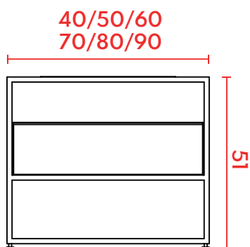
VISTA FRONTAL
