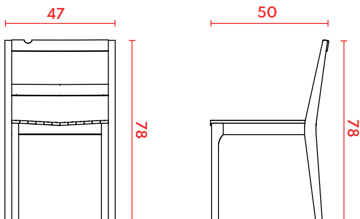
VISTA FRONTAL
